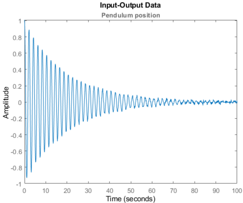
Figure 2: Angular position of the pendulum (output).
