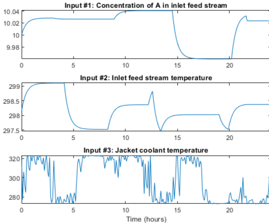
Figure 2: Estimation data set inputs to a CSTR.
